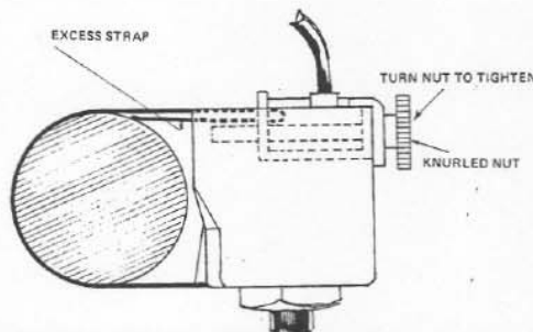
FIGURE 1 – 367 Switch
